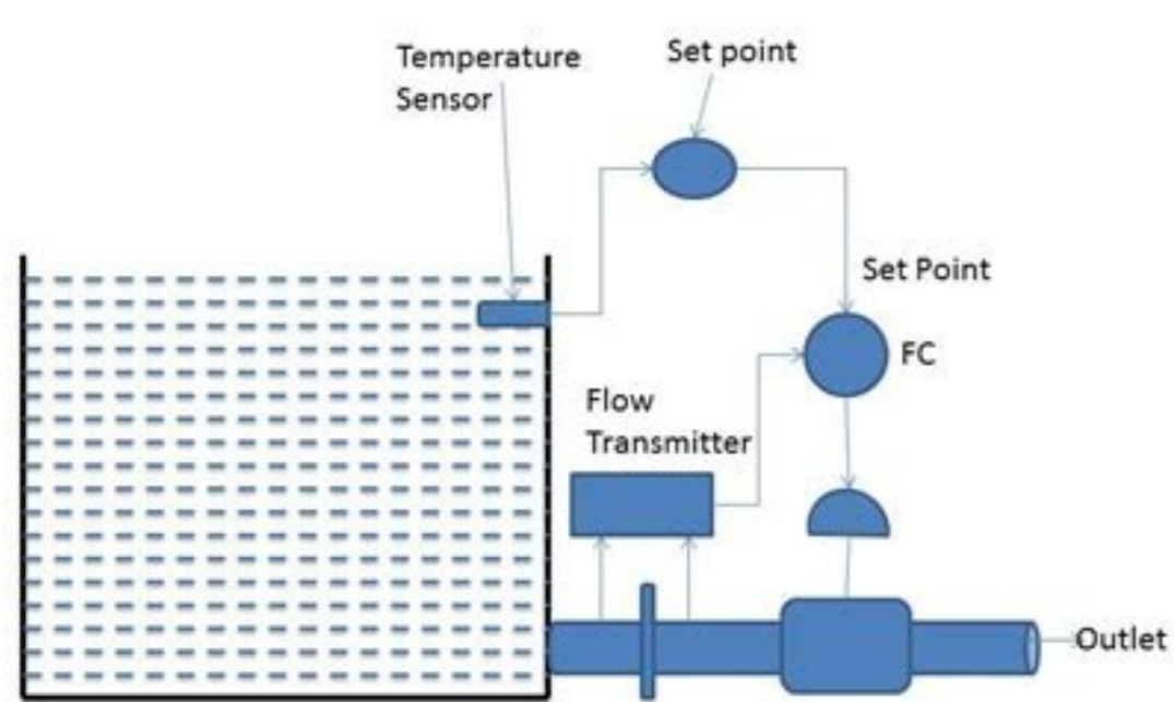
Example - Cascade Control System
